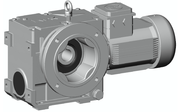
İRSDFM ...-FL
